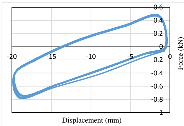
Figure 6: Displacement- Force graph of FFFfluid under dynamic load.
