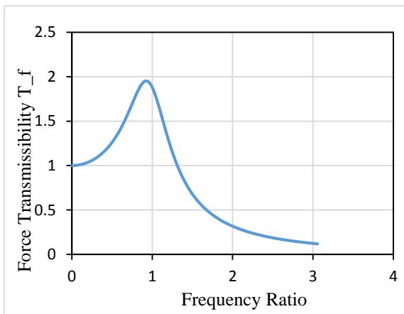
Figure 8: Transmissibility of FFFfluid isolator.
