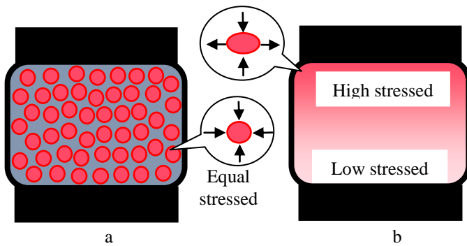
Figure 2: Foam under compression load: (a) FFFluid, (b) dry foam
