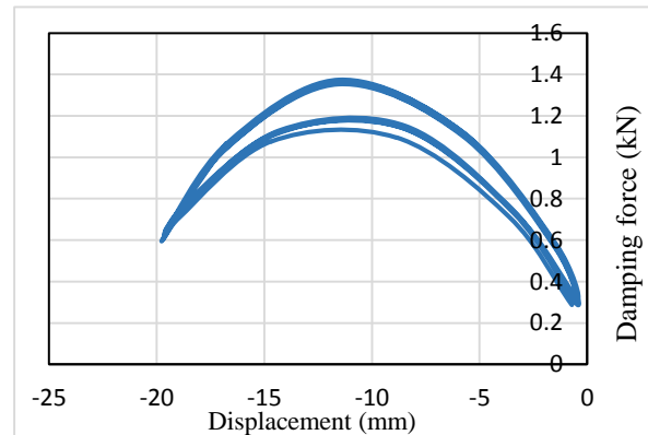
Figure 7: Displacement- viscous force graph of FFFfluid under dynamic load
