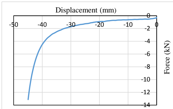
Figure 5: Displacement- Force graph of FFFfluid under static load.
