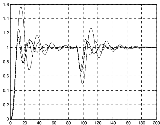
Fig. 6b. Responses of (9) for L=0.5 ; FPIC(—),STFPIC(— ·),NF-STFPIC(- ·).
