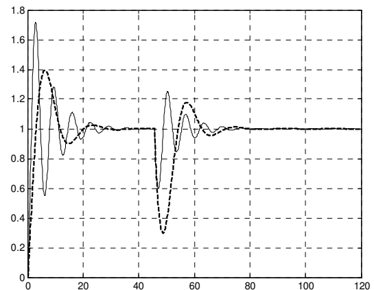
Fig. 4d. Responses of (7) for L=0.2 ; ZNPIDC(—) and TLPIDC(– ·).
