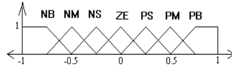
Fig. 2. MFs of e_N , \Delta e_N and \Delta u_N .
