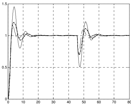
Fig. 4a. Responses of (7) for L=0.2 ; FPIC(—);STFPIC(– –),NF-STFPIC(– ·).
