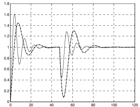
Fig. 4c. Responses of (7) for L=0.2 ; ZNPIC(—) and TLPIC(– ·).
