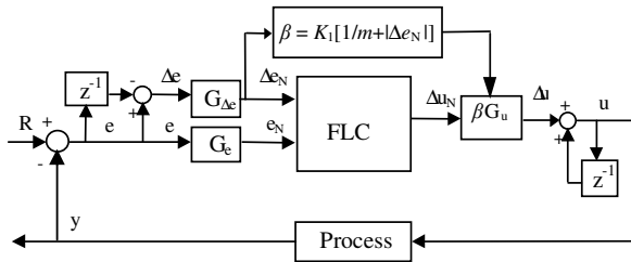
Fig. 1. Block Diagram of the proposed NF-STFPIC
