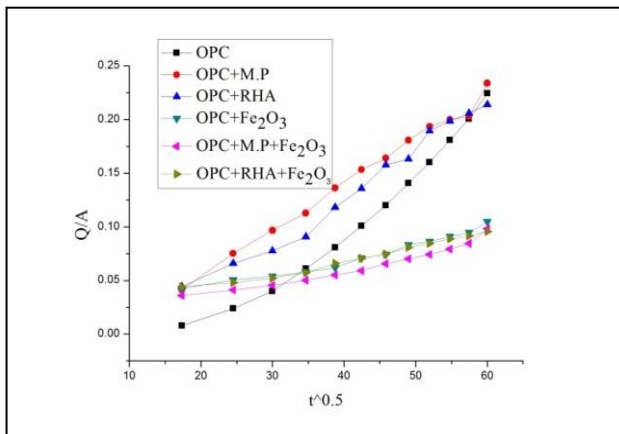
Sorptivity test for control vs Nano Fe 2 O 3
