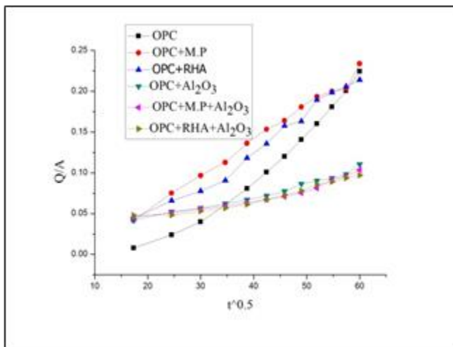
Sorptivity test for control vs Nano alumina system
