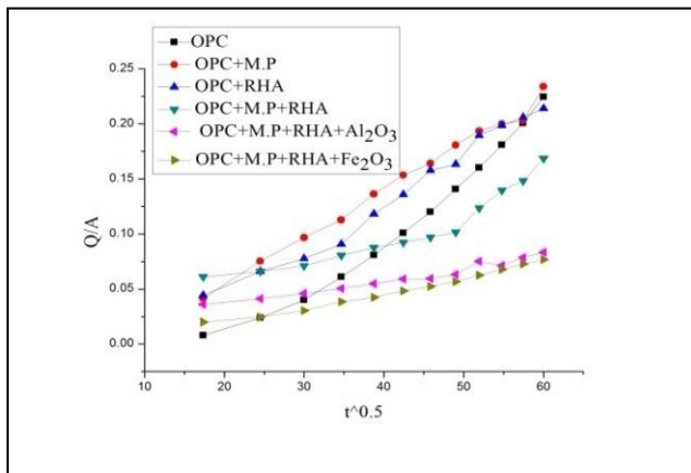
Sorptivity test for single vs combine system
