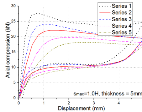
Figure 3. Load-displacement responses of selected SMA washers.
