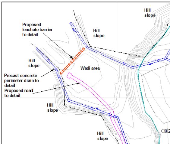
Figure 4: The proposed site of the subterranean leachate barrier.
