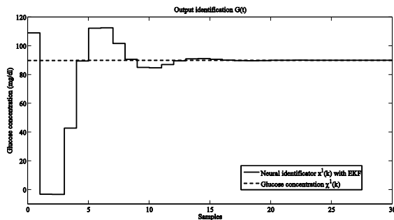
Figure 1. Output identification: glucose concentration x'(k) (dashed line); variable x^l(k) identification with the EKF method (bold line).
