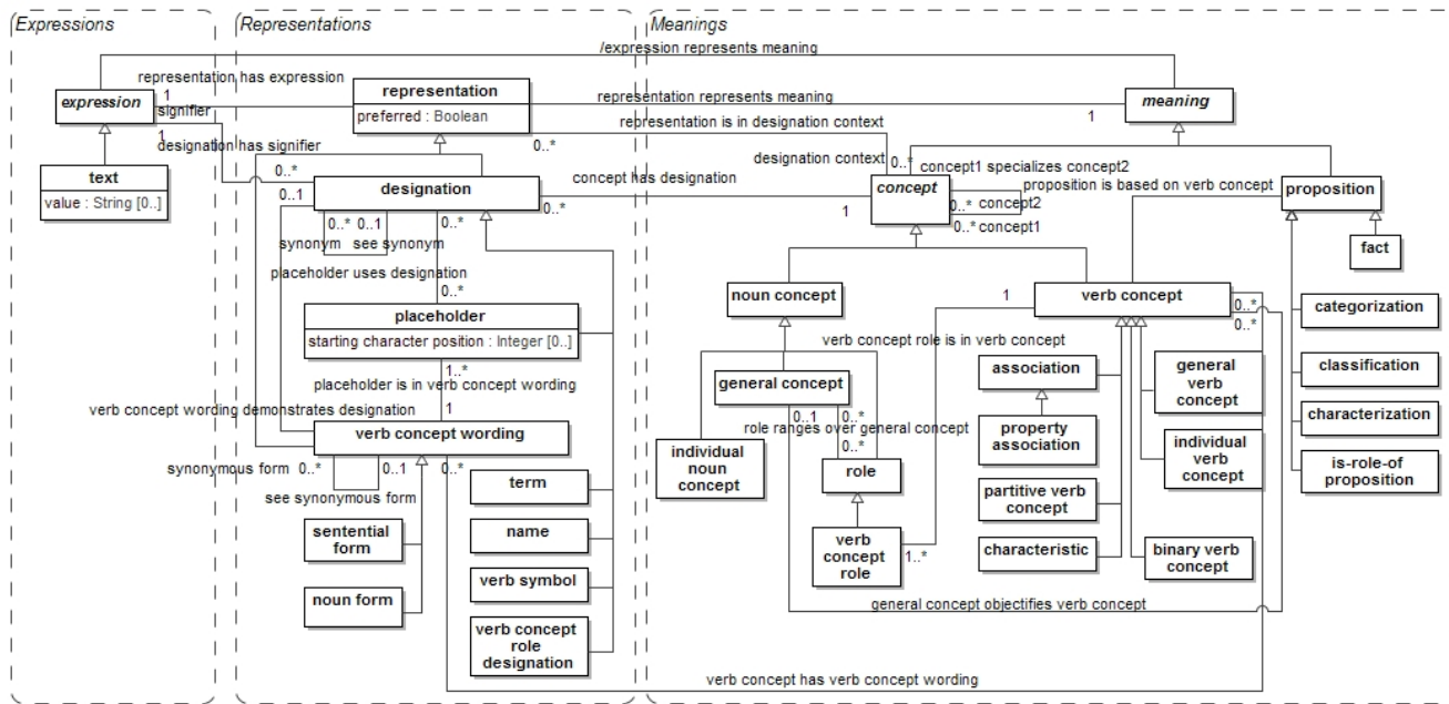
Figure 1. SBVR metamodel for SLOL, relating meanings, expressions and representations (adapted from[1])
