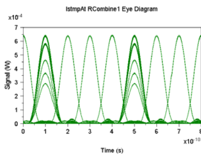
Fig.3: Eye Diagram without Fuzzy Controller after combiner
