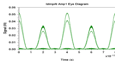
Figure 6: Eye diagram with Fuzzy Controller after encoder
