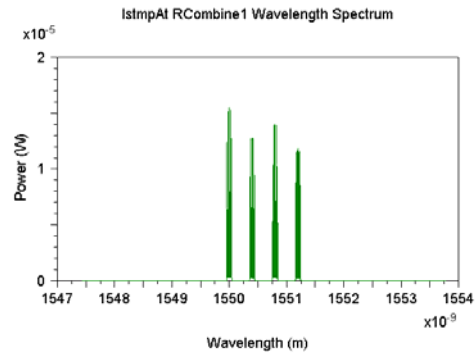
Figure 4: Wavelength spectrum without fuzzy controller
