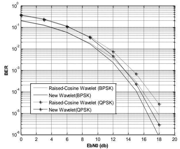
Figure 5: Comparison of ideal-filter wavelet with Root Raised Cosine Wavelet ( \beta=1/3 ) over multipath channel with AWGN for \varphi_2 .
