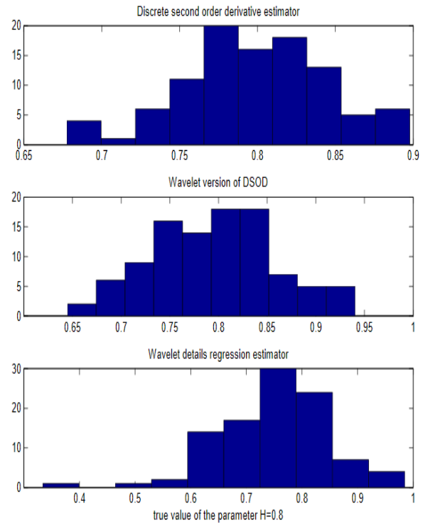
Figure 1. True values of the Hurst exponent for set A
