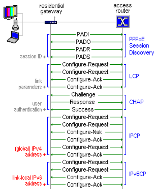
Figure 3. PPP link setup
