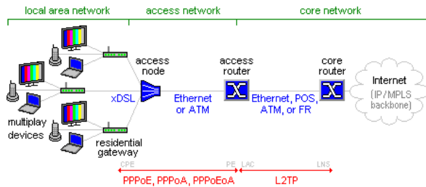
Figure 2. PPP in the Context of Broadband Access Networks
