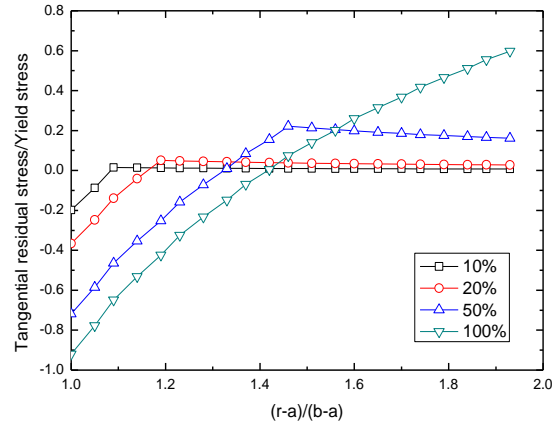
Figure 3. Theoretical tangential residual stress distributions in an autofrettaged pipes.
