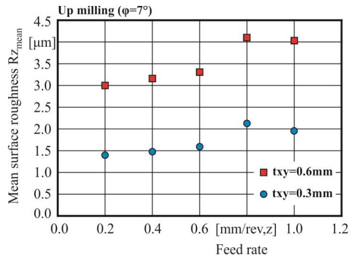
D20, z=1 , Carbide, Al7075-T6 t_z=0.3\text{mm} , t_{xy}=0.3\text{mm} , n=5000\text{rpm}
