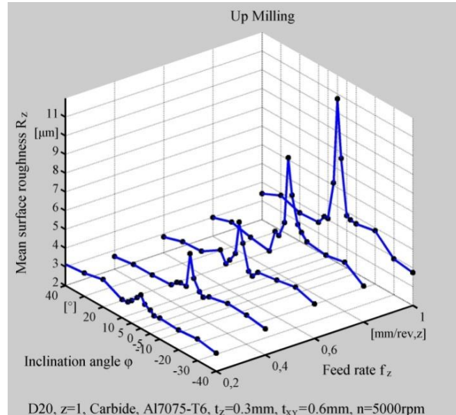
Figure 3. Mean Surface Roughness in up milling with t_z=0.3\text{mm} and t_{xy}=0.6\text{mm}
