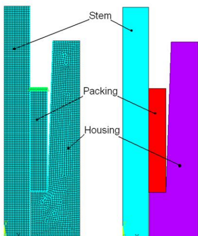
Figure 3. FE model of a packed stuffing box with a tapered housing
