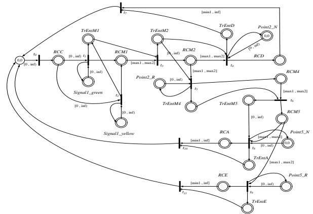
Figure 7. Track Circuit Timed-Arc Petri Net Model for Trains that Entering the Station form C.
