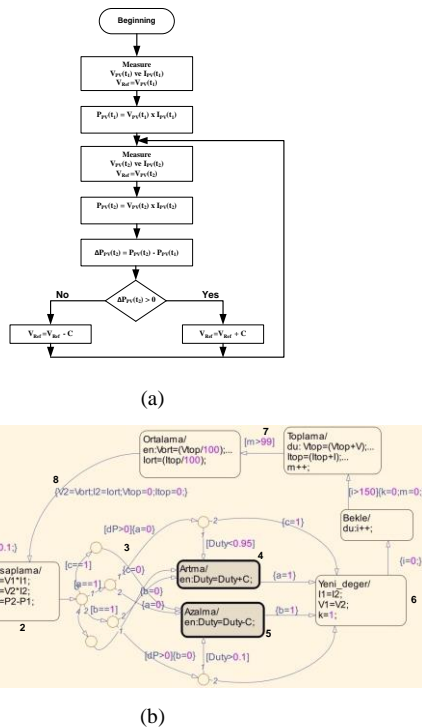
Figure 4. P&O algorithm flowchart (a) and Matlab/Stateflow model (b)
