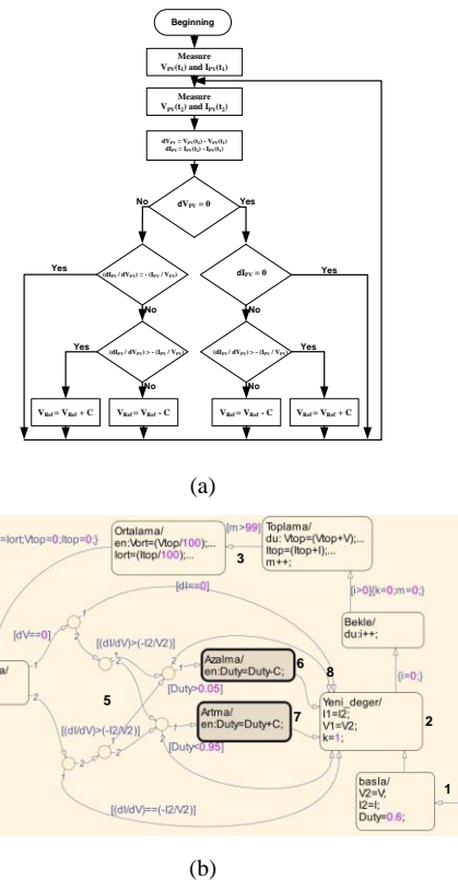
Figure 5. IC algorithm flowchart (a) and Matlab/Stateflow model (b)
