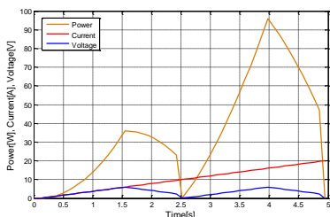
Figure 8. SC Current, voltage and power variation
