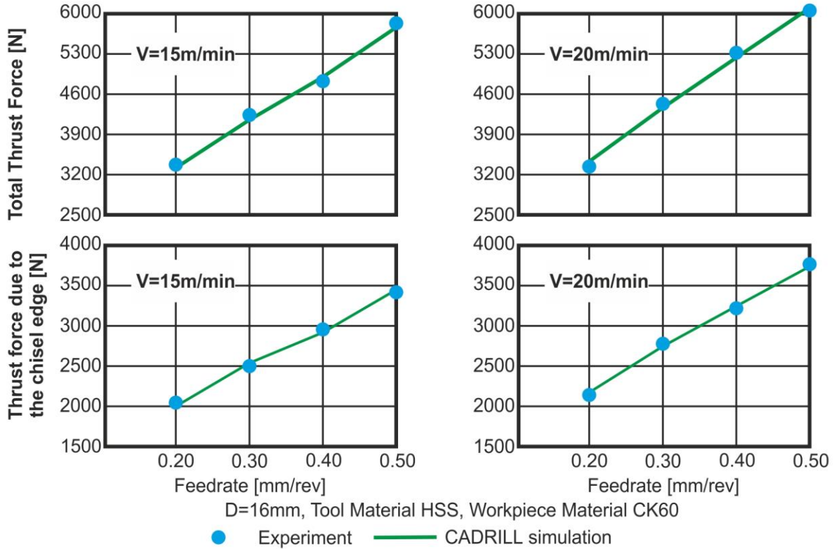
Figure 4. Evaluation of CADRILL using a D=16mm twist drill
