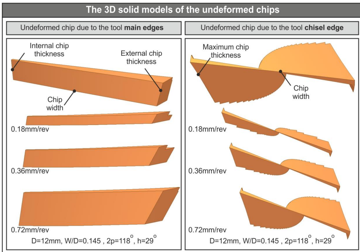
Figure 2. 3D solid models of the main edges and chisel edge undeformed chips
