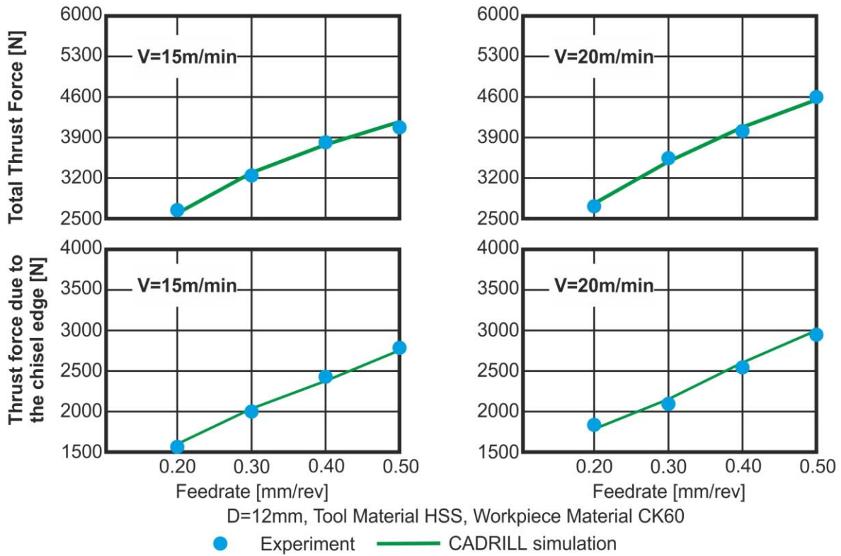
Figure 3. Evaluation of CADRILL using a D=12mm twist drill
