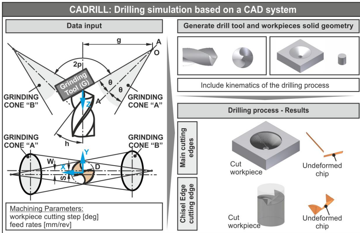
Figure 1. Drilling process simulations using a CAD system
