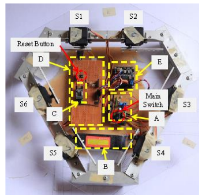
Figure 4: Fixed Base of Parallel Manipulator
