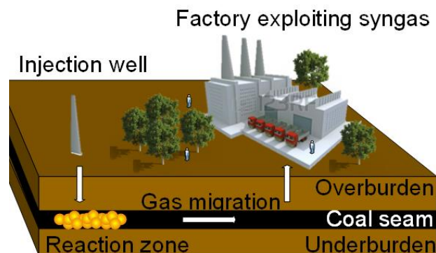
Figure 1. Example of the UCG process schema.
