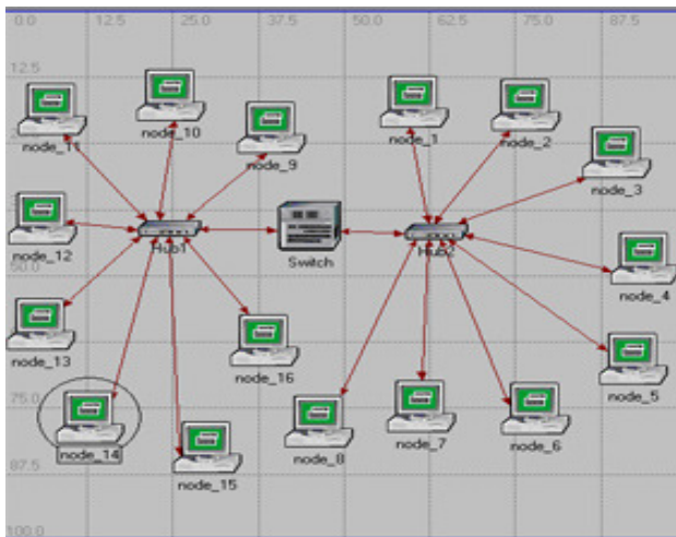
Figure 1. Campus network under 10BaseT with two hubs
