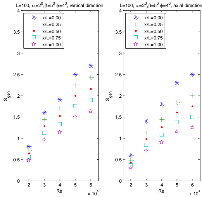
Figure 3. Local dimensionless entropy generation with the Re number
