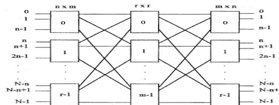
Figure 1. A Basic General Clos Interconnection Network
