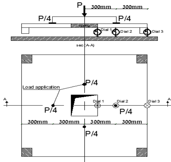
Figure 6. Shows dimensions of typical test RC slabs and arrangement of dial gauges of group (B)
