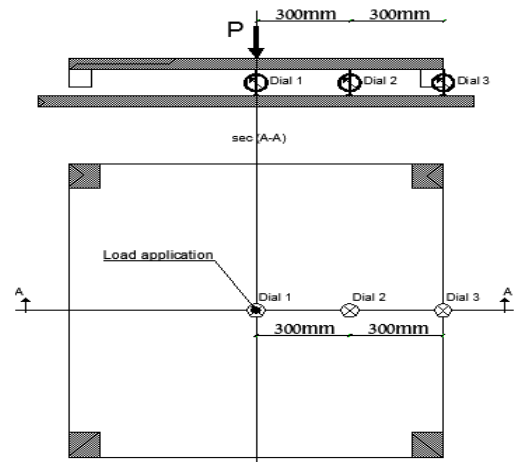
Figure 3. Shows dimensions of typical test RC slabs and arrangement of dial gauges of group (A)
