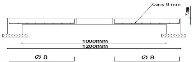
Figure 7. Shows Reinforcement of typical test RC slabs of group (B)
