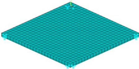
Figure 5. 3D finite element meshes for RC slabs of group (A).
