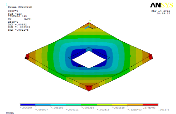
Figure 12. Deflection Contour lines for RC slab HSO5 in m using ANSYS
