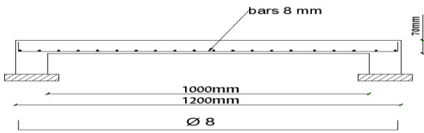
Figure 4. Shows Reinforcement of typical test RC slabs of group (A)
