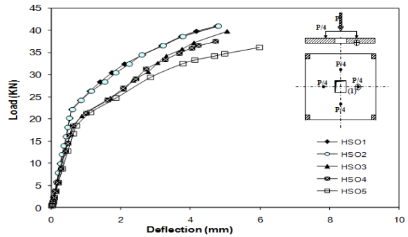
Figure 11. Comparison between Load - Deflection Curves of all RC Slabs of group (B) at Point (1) by ANSYS.
