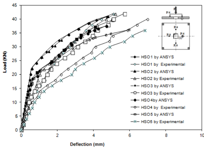
Figure 14. Comparison between experimental and analytical values from ANSYS for Load -Deflection Curves of all RC Slabs of group (B) at Point (1).
