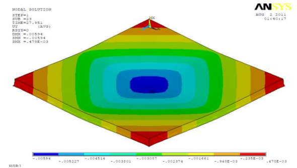
Figure 10. Deflection Contour lines for RC slab HSR1 in m using ANSYS
