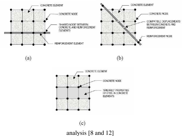
Figure 2. Models for reinforcement in reinforced concrete; (a) Discrete; (b) Embedded; (c) Smearred [12]
