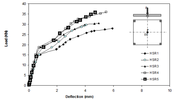
Figure 9. Comparison between Load - Deflection Curves of all RC Slabs of group (A) at Point (1) by ANSYS.
