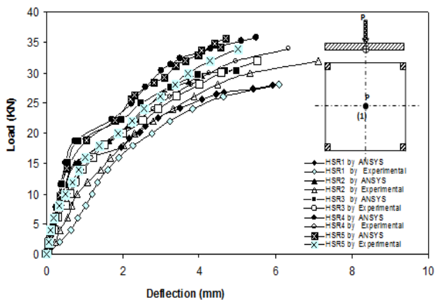
Figure 13. Comparison between experimental and analytical values from ANSYS for Load - Deflection Curves of RC Slabs of group (A) at Point (1).
