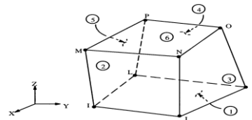
Figure 1. Solid 65 – 3-D reinforced concrete solid element used for concrete
