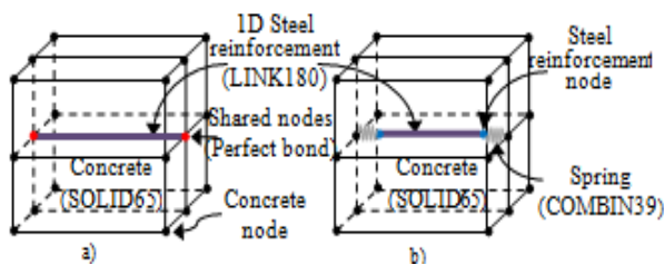
Figure 5. Reinforcement and bond-slip modeling details of a) LN-PB b) LN-SPR
