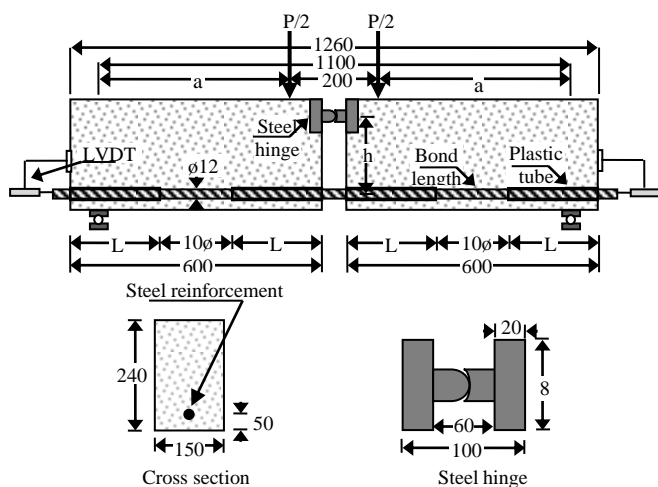
Figure 2. Beam bending test according to RILEM [24].
