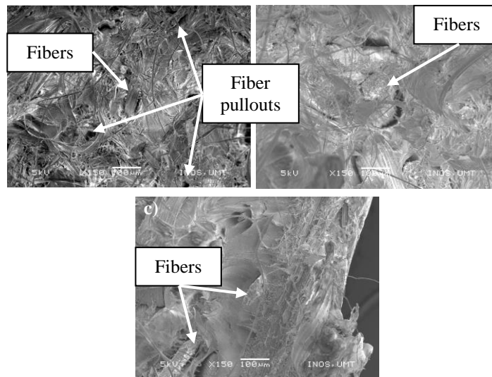
Figure 4. SEM micrograph of tensile fracture surface of a) AG/HDPE, b) AG/HDPE with addition of PE-g-MA and c) AG/HDPE with addition of ECO composites at 15 wt% under x150 and magnification.
