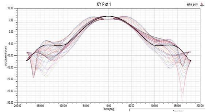
Fig 9: Rectangular gain plot for PPy patch
