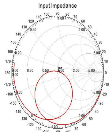
Fig 7: Input impedance of PPy structure
