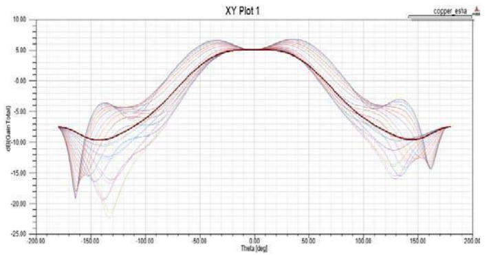
Fig 10: Rectangular gain plot for Cu patch
