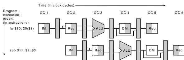
Figure 4: Five Stage Pipelining
