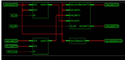
Figure 14: RTL Schematic of MIPS Instruction Decode Unit obtained by Synthesis using Xilinx 9.2i.
