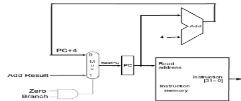
Figure 5: Instruction Fetch unit
