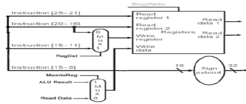
Figure 6: MIPS Instruction Decode Unit
