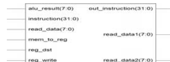
Figure 13: Block diagram of MIPS Instruction decode Unit obtained by Synthesis using Xilinx 9.1.
