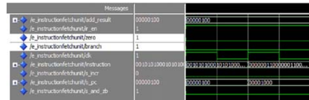
Figure 12: Waveforms of MIPS Instruction fetch Unit obtained by Simulation using Modelsim 6.3f.
