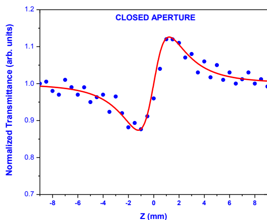
Fig. 3: Closed aperture measurements (at 532 nm) of permethylazine. “Symbols” represent experimental data and “solid lines” represent theoretical fit.
