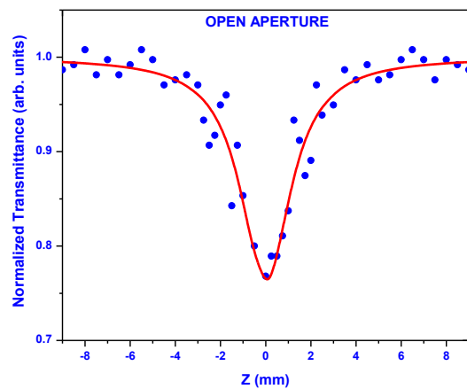
Fig. 2 Open aperture measurements (at 532 nm) of permethylazine. “Symbols” represent experimental data and “solid lines” represent theoretical fit.
