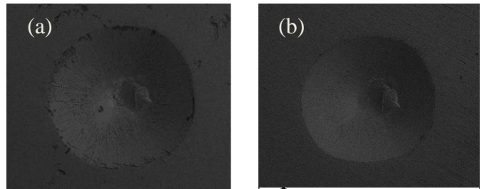
Fig.4 Rockwell Indentation Test for Adhesion of (a) MS PVD TiN coated (b) MS Duplex (PN+ PVD TiN coated)
