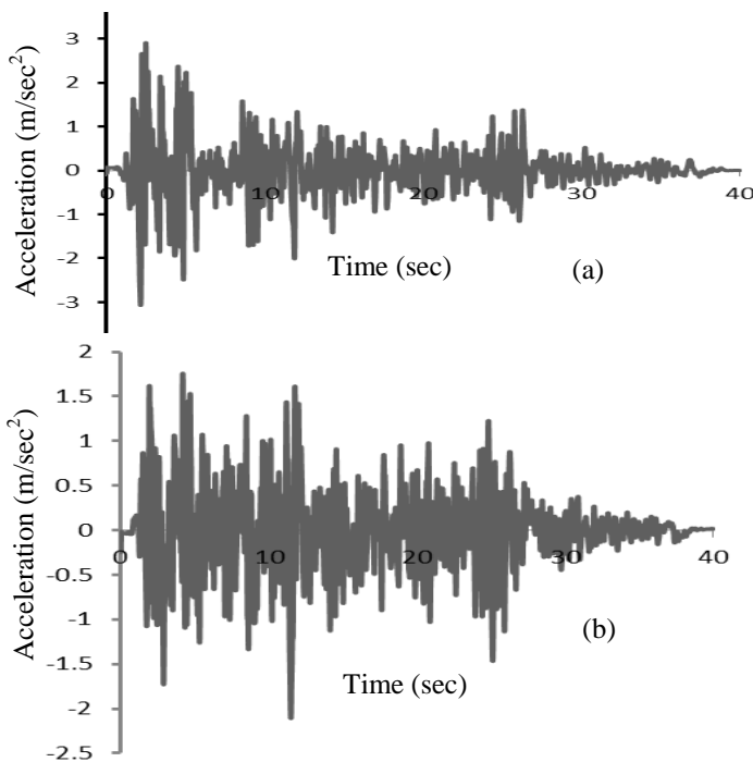
Figure 1. Ground Motions Considered (a) PGA 0.313g; (b) PGA 0.215g.
