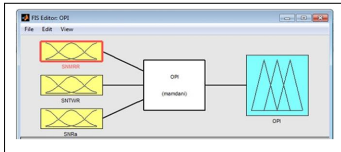
Figure 6. Fuzzy relation
