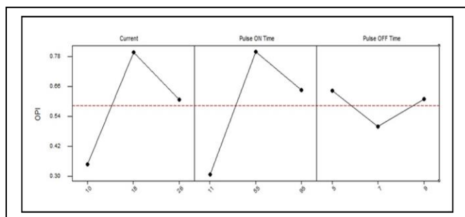
Figure 12. OPI graph
