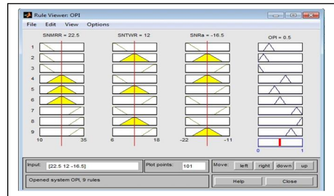
Figure 11. Fuzzy output
