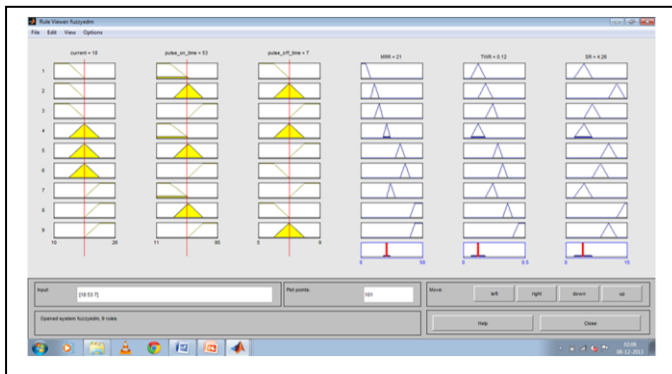
Figure 2. Rule viewer
