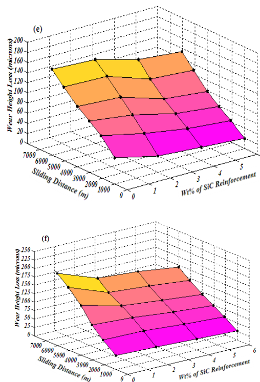
Figure 4 (a) to (f). Prediction for the relationship of wear height loss as a function of sliding distance and wt% of SiC reinforcement at a constant applied load (10 to 60N).
