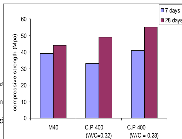
Bar Chart: 1 comparison of compressive strength vs water cement ratio of CERAPLAST- 400 for M 40
