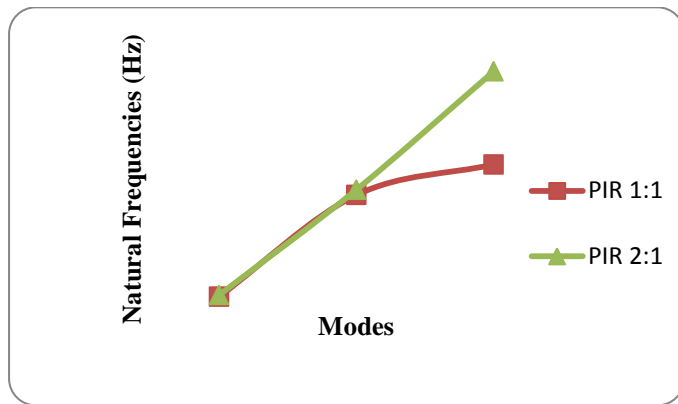
Figure 14: Comparison of natural frequencies of PIR foam of 1:1 and 2:1 corresponding to modes from experimental test
