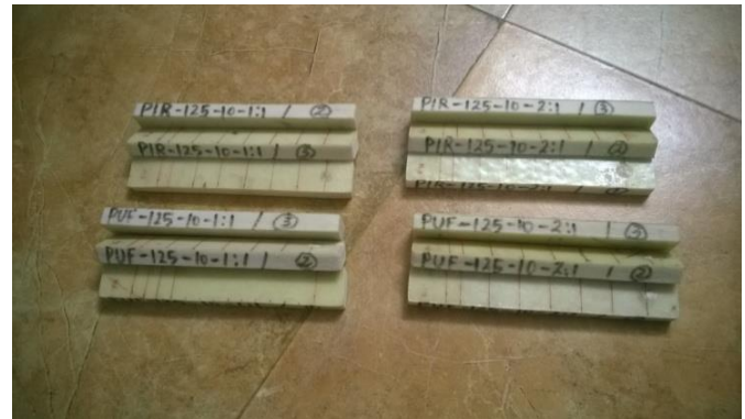
Figure 3: Both PUF and PIR 125 Kg/m 3 of 1:1 and 2:1 weight ratio sandwich specimens for testing
