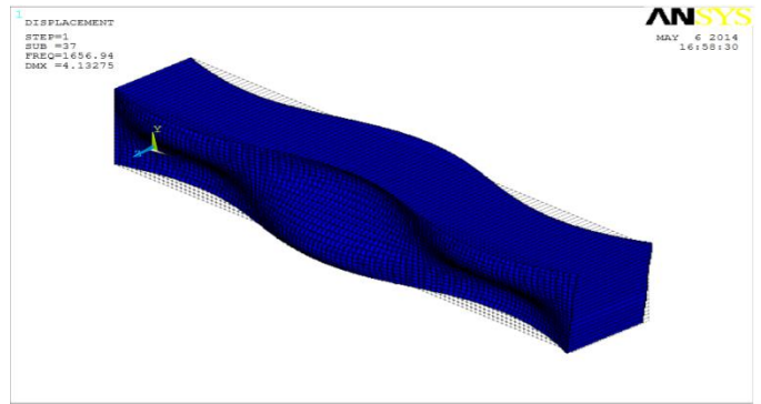
Figure 13: Mode 3 shape of PIR 2:1, f_3 = 1656.94 Hz
