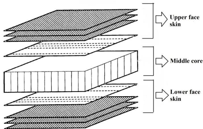
Figure 1: Typical Sandwich Structure
