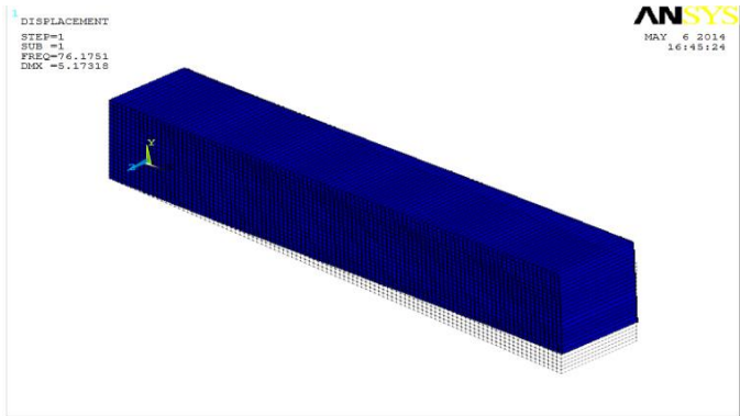
Figure 11: Mode 1 shape of PIR 2:1, f_1 = 76.17 Hz
