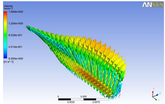
Figure 10. Velocity vector at 60° sharp bend section
