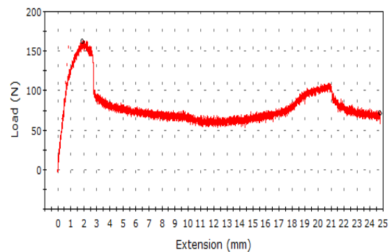
Figure.7.Double Lap Shear-Load deflection plot for PUF - 250
