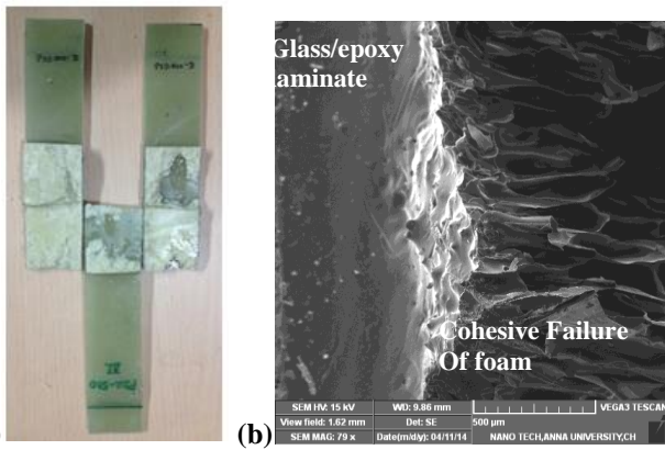
Fi Figure.4 (a)Cohesive- Adhesive failure in PUF 500 (b)SEM of Double Lap Shear Cohesive Failure - PUF 125
