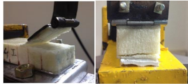
Figure.5: Peel Failure on top laminate Figure.6: Peel failure on bottom laminate
