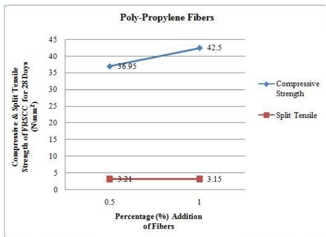
Fig.4. Compressive & Split Tensile strength of PP fibers for 28 Days
