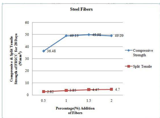
Fig.3: Compressive & Split Tensile strength of Steel fibers for 28 Days
