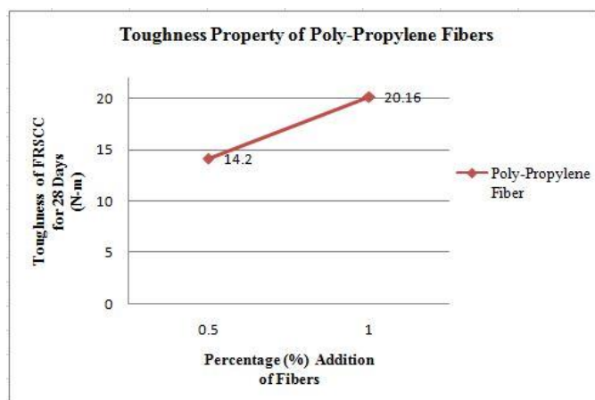
Fig.8: Toughness property of PP FRSCC for 28 Days.
