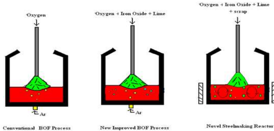
Fig.1 Schematic diagram of different oxygen steelmaking processes
