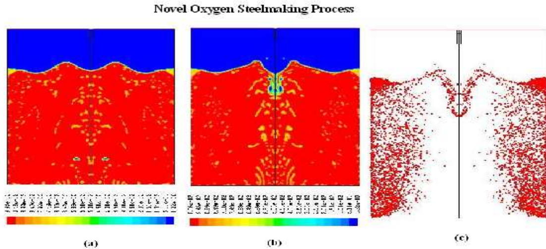
Fig.4 Multiphase Plot Novel Oxygen steelmaking Process at (a) Conventional with stirring (b) New oxygen steelmaking process with stirring (c) Discrete phase particle position with stirring.
