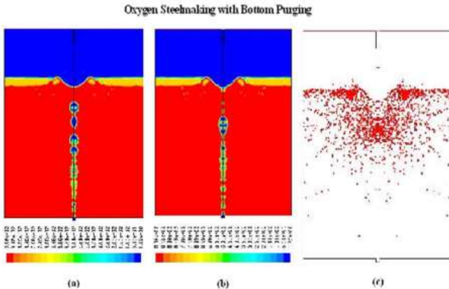
Fig.3 Multiphase Plot (a) Conventional (b) New Oxygen Steelmaking Process (c) Discrete phase plot of New Oxygen steelmaking Process with bottom purging
