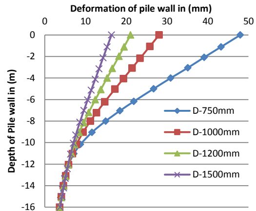
Fig. 7 Effect of Diameter of Pile on deformation of Pile wall
