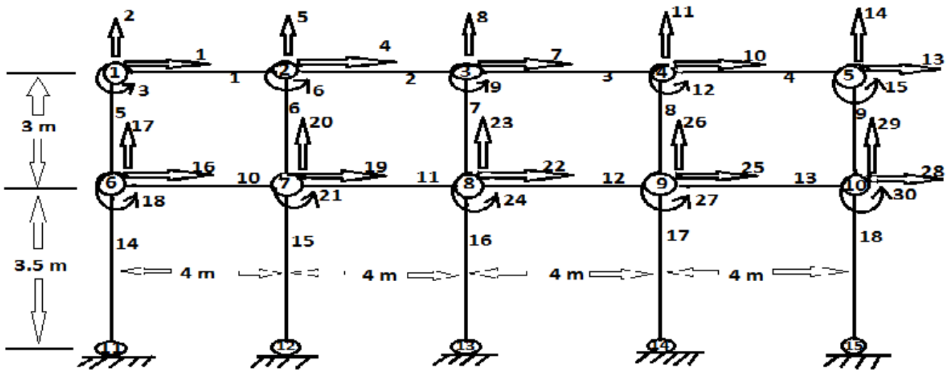
Fig. 1 – 4 Bay 2 Storied 2D Frame
