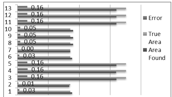
Bar chart-3: Error in Cross-sectional Area (3D Frame):
