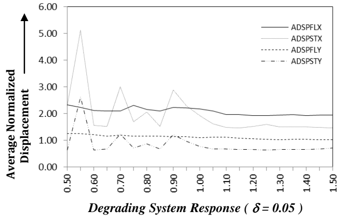
Fig. 3: Average normalized displacement response of structural systems with T_1=0.1s , e_x/D=0.2 and e_y/D=0.05
