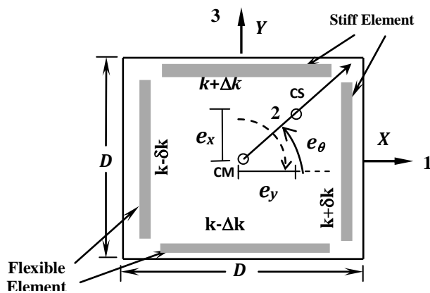
(b) Bi directional Eccentric system
