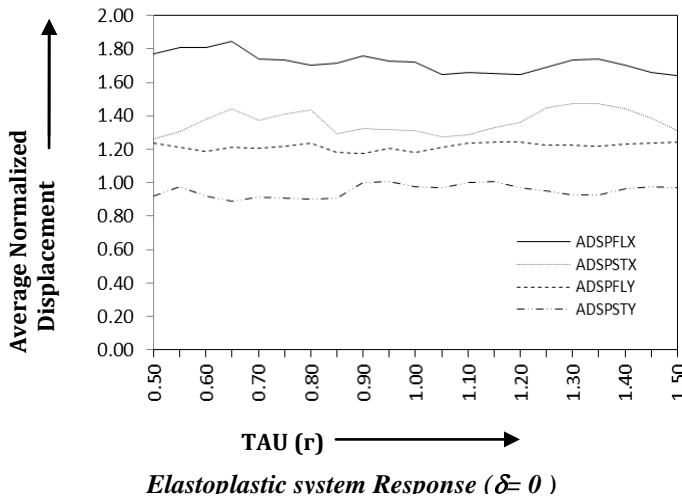
Fig.2: Average normalized displacement response of structural systems with T_1=0.1s , e_x/D=0.2 and e_y/D=0.1
