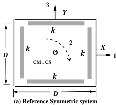
(a) Reference Symmetric system
