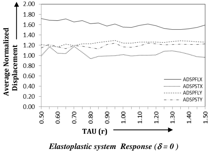
Fig. 3: Average normalized displacement response of structural systems with T_1=0.1s , e_x/D=0.2 and e_y/D=0.05
