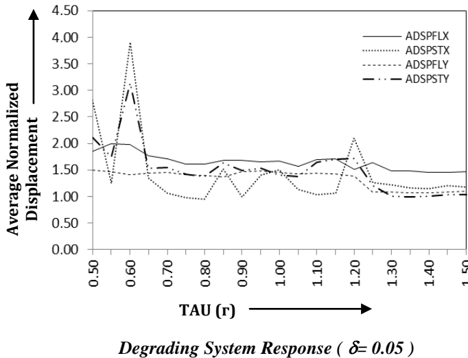
Fig.2: Average normalized displacement response of structural systems with T_1=0.1s , e_x/D=0.2 and e_y/D=0.1
