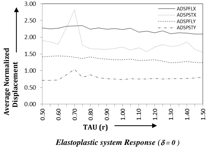
Fig.4: Average normalized displacement response of Structural systems with T_1=0.1s , e_x/D=0.2 and e_y/D=0.2
