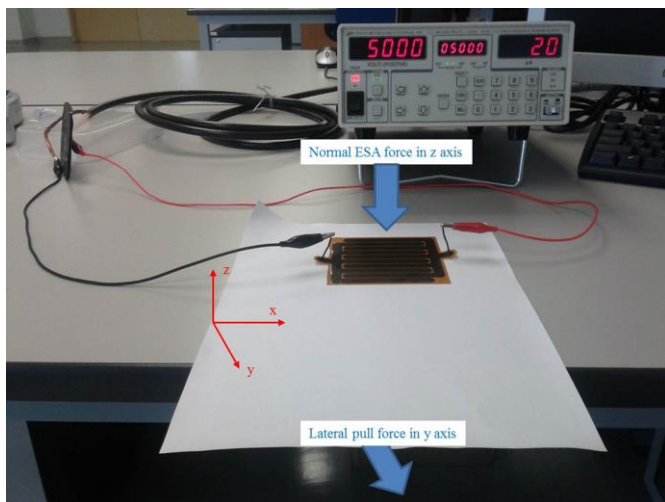
Fig. 3. Pull experiment with FPC electrostatic device, shown actuated at 5kV.
