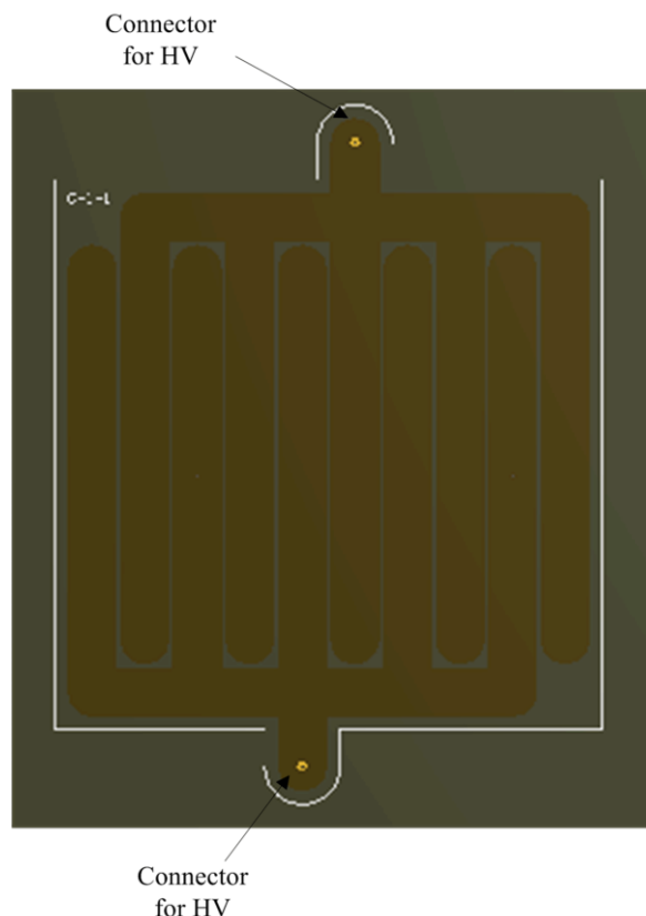
Fig. 2. Electrostatic device with interdigitated electrode pattern.
