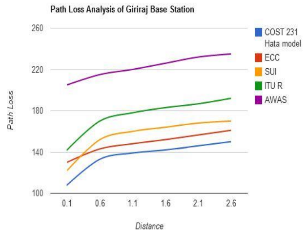
Fig 3(c) Path Loss Analysis of GRJ Base Station
