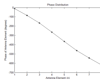
Figure 7(c): Phase Distribution
