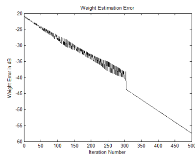
Figure 7(d): Weight Error
