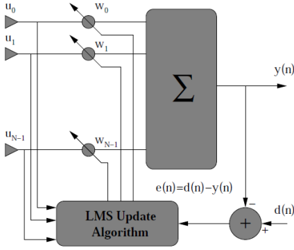
Figure 5: LMS algorithm [3]
