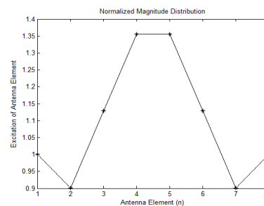
Figure 7(b): Magnitude Distribution
