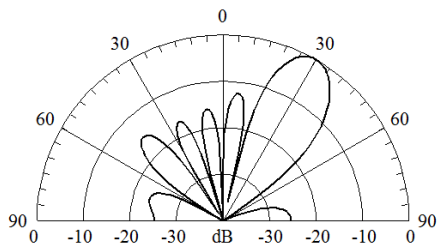
Figure 8(a): Radiation Pattern
