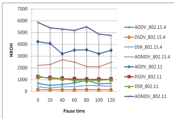
Fig – 2: NROH vs. Pause time
