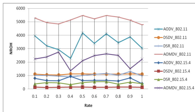
Fig - 6 NROH vs. Rate
