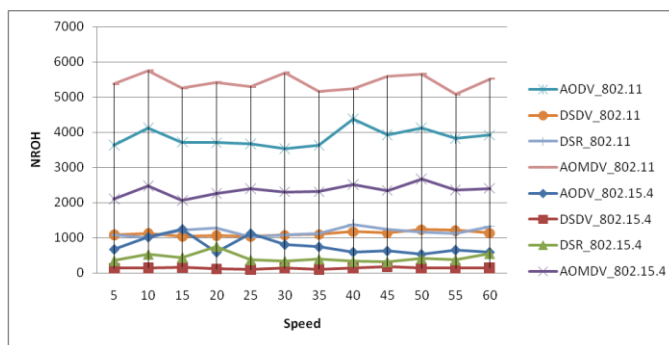
Fig – 4: NROH vs. Speed
