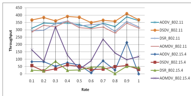
Fig – 5: Throughput vs. Rate
