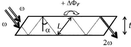
Figure 1. Phase matching technique using Total Internal Reflection in parallel semiconductor slab for second harmonic generation scheme.
