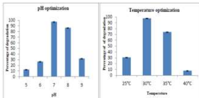
Fig. 2 Optimization of pH and temperature: optimum pH was pH 7 and temperature was 30°C
