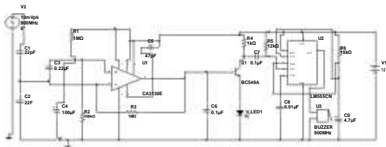
Fig 2.The developed sniffer circuit
