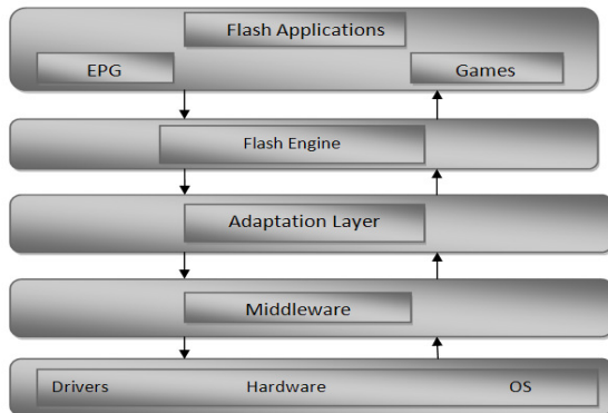
Figure 2. Set top box flash architecture.
