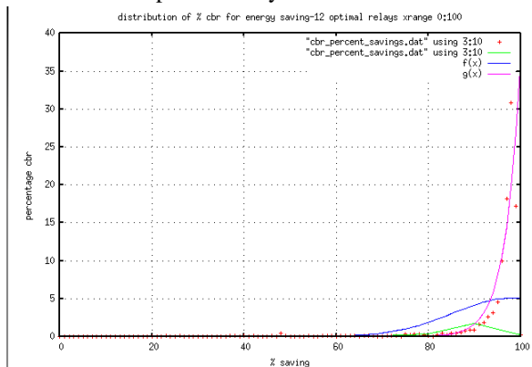
Fig 27: Trends of energy savings– 12 opt relays.
