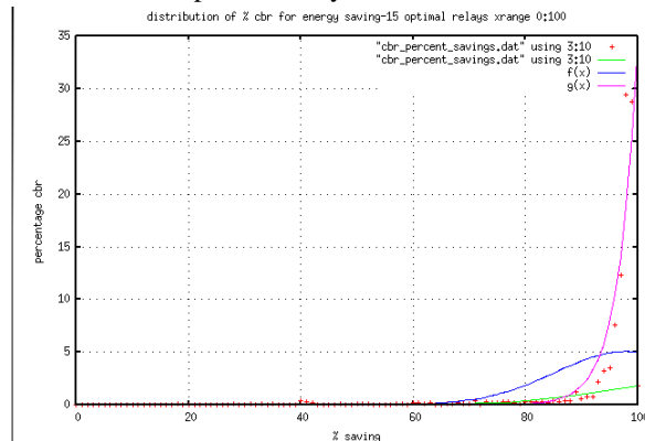
Fig 30: Trends of energy savings– 15 opt relays.
