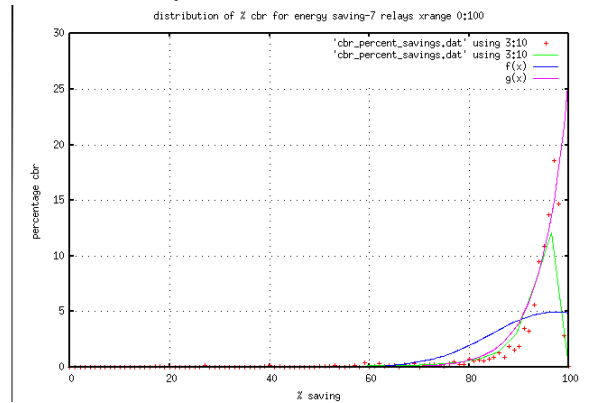
Fig 7: Savings achieved by cbrs- 7 relays
