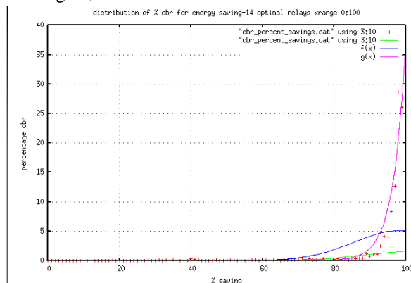
Fig 29: Trends of energy savings– 14 opt relays.
